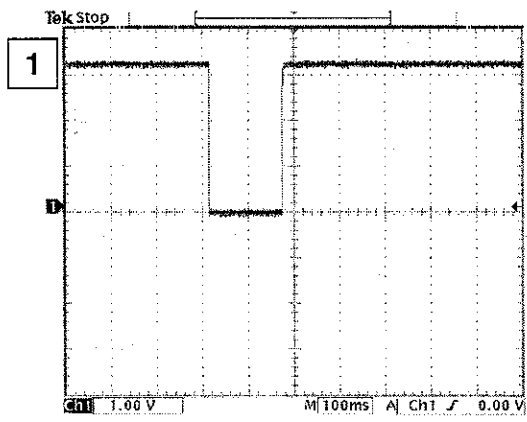
Fig.1 <Tact Switch pulse>
