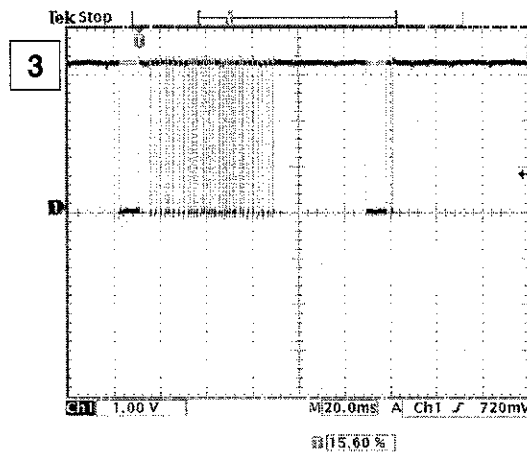
Fig.3 <IR receiver Pulse>
